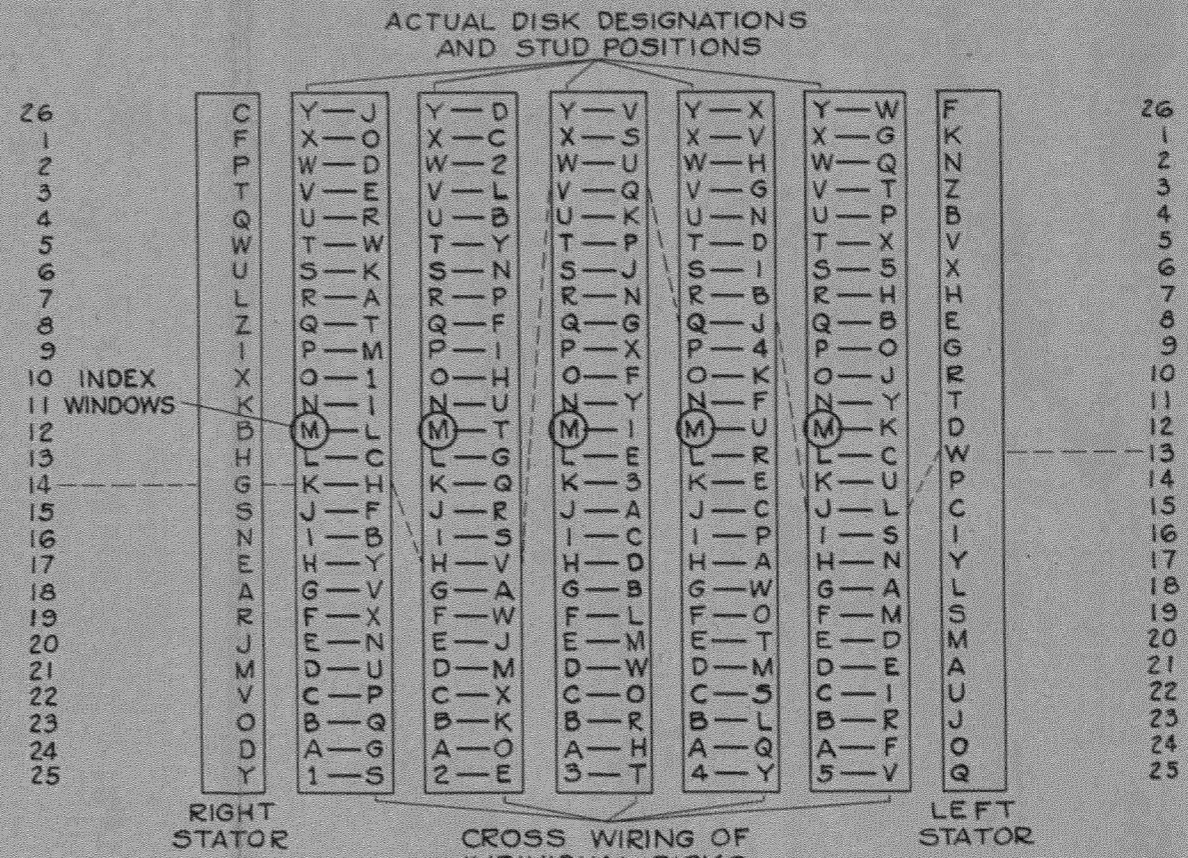
FIG. 17 CROSS WIRING OF INDIVIDUAL DISKS CIPHER DISK CONNECTION
