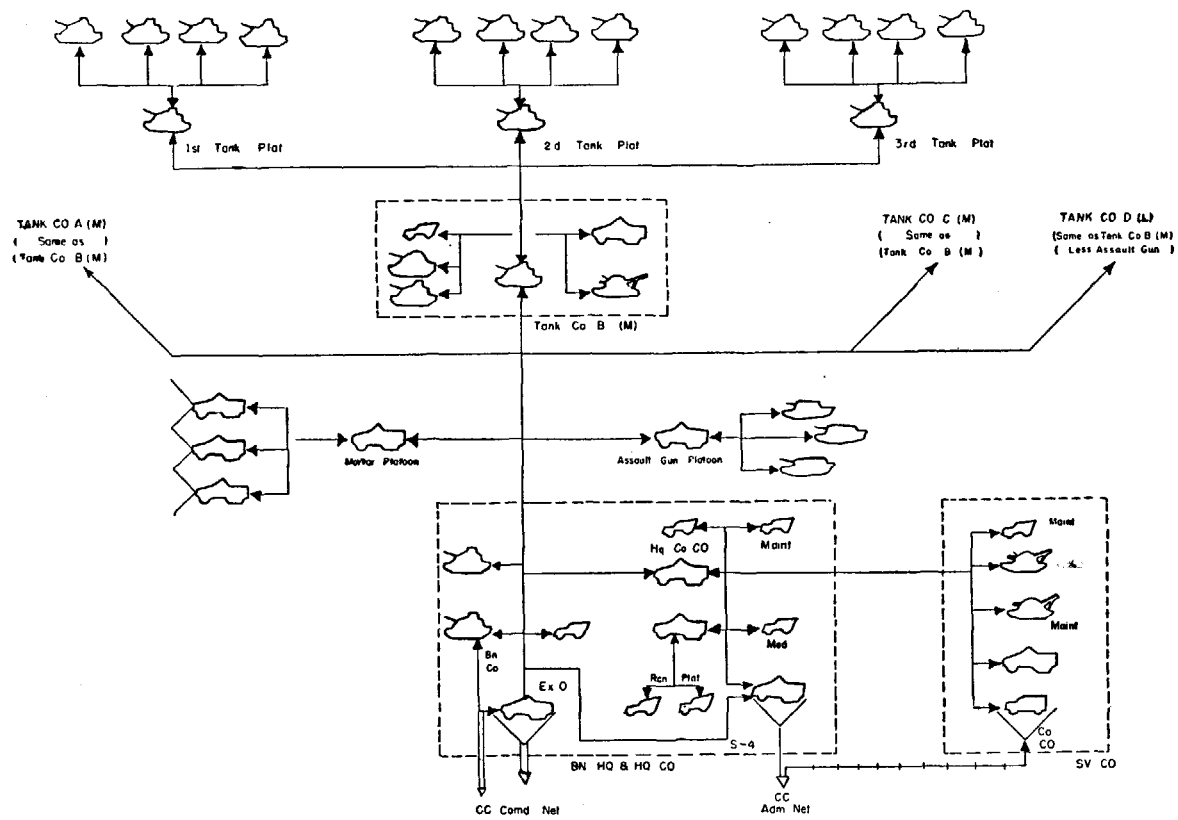
Figure 8. Type radio nets, tank battalion.
