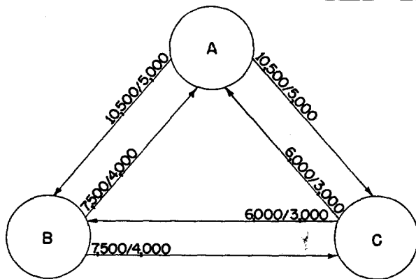
Figure 25. The net uses the complex-sending system.
