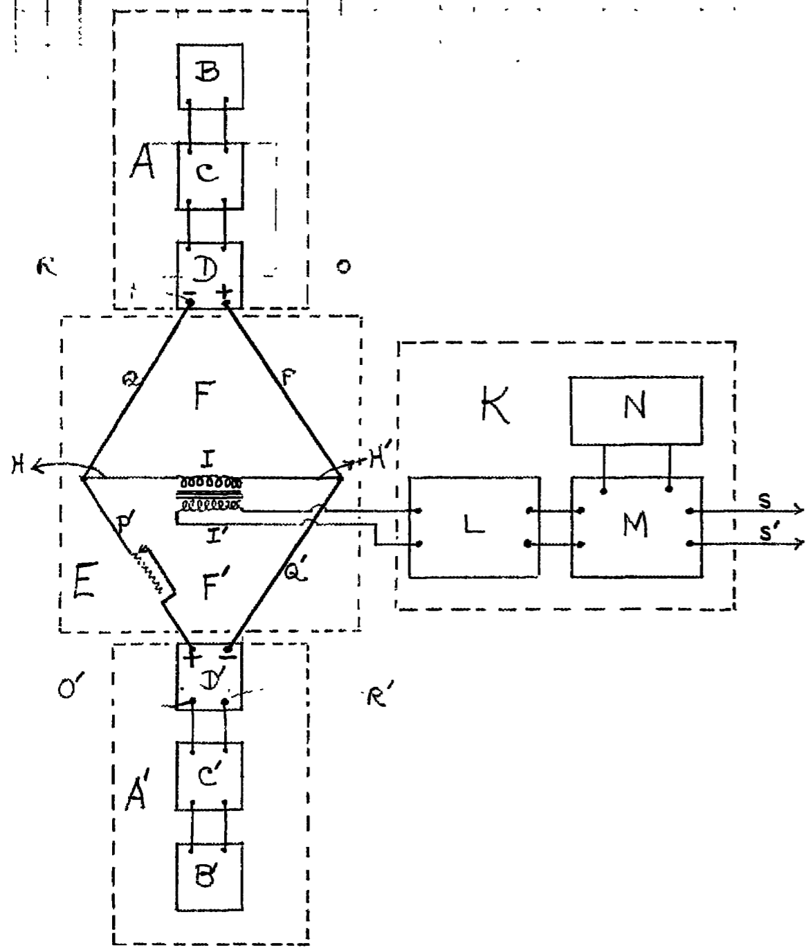
FIG 1 TRANSMIT
