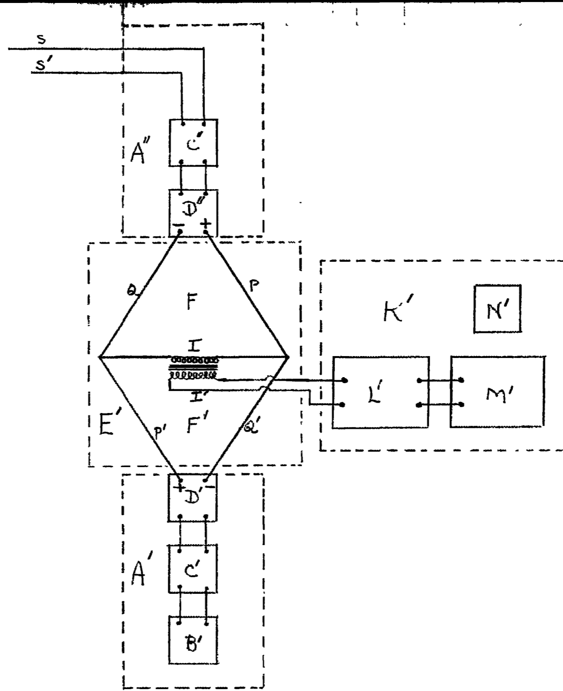
FIG 2 RECEIVE
